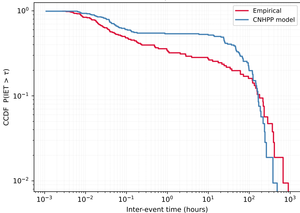
User 185880661 - Empirical vs CNHPP model
